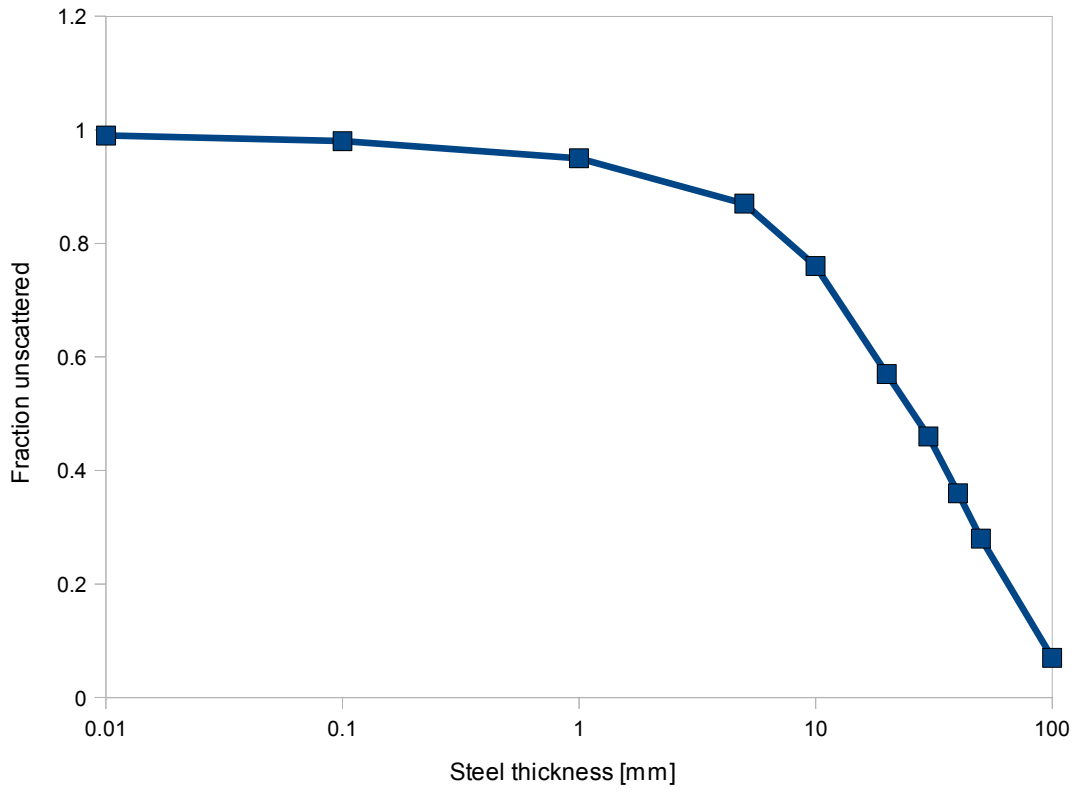
ATF Laser-wire photons through steel
