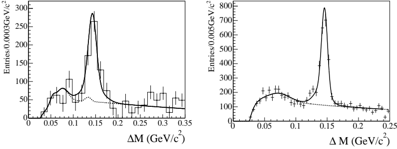
Figure 3: f_{D_s} analysis: (left) \Delta M distribution for D_s^+ \rightarrow \mu^+ \nu_\mu events after the tag side-bands and the electron sample are subtracted. The solid line is the fitted signal + background distribution, while the dotted line is the background distribution alone. (right) \Delta M distribution for D_s^+ \rightarrow \phi \pi^+ events after the tag side-bands are subtracted. The solid line is the fitted signal + background distribution, while the dotted line is the background distribution alone.
