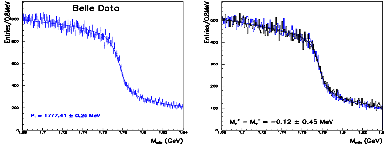
Figure 6: \tau mass analysis: (left) pseudo-mass distribution ( M_{min} ) for events selected in the \tau^\pm \rightarrow 3\pi^\pm\nu_\tau decay mode. The point with error bars data and the solid line is the result of the fit with the function in Equation 6. (right) pseudo-mass distribution ( M_{min} ) for \tau^+ and \tau^- decays in the 3\pi^\pm\nu_\tau decay channel. The solid lines are the results of the fit using the function in Equation 6.
