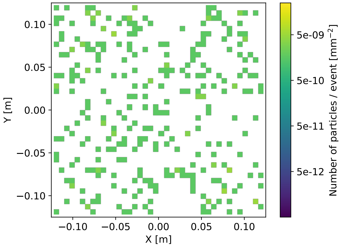
MuonP flux at FASER IP
