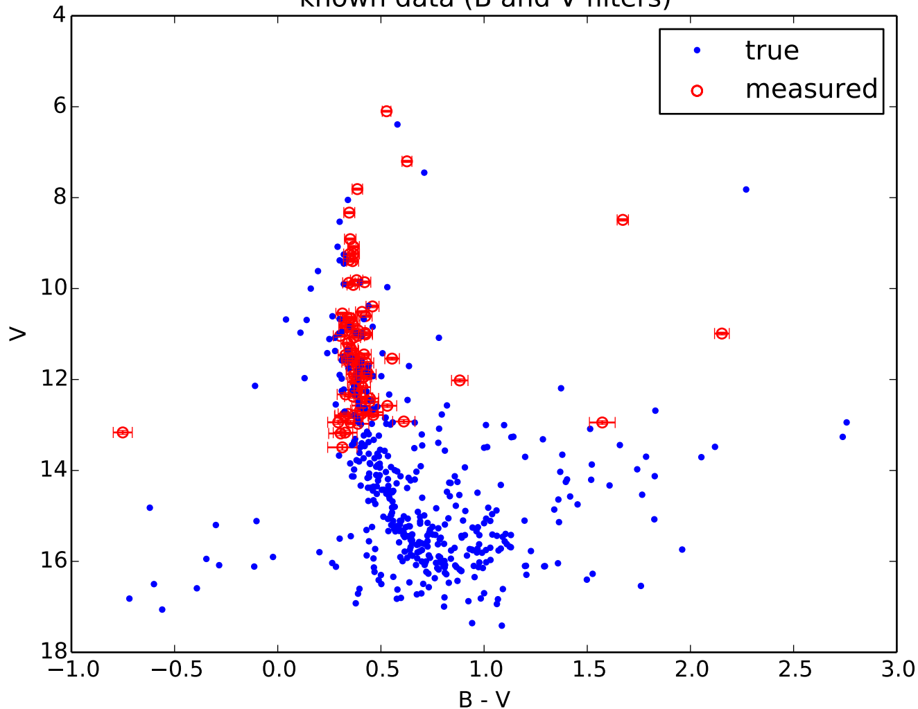
HR diagram for real Double Cluster, comparing measured and known data (B and V filters)
