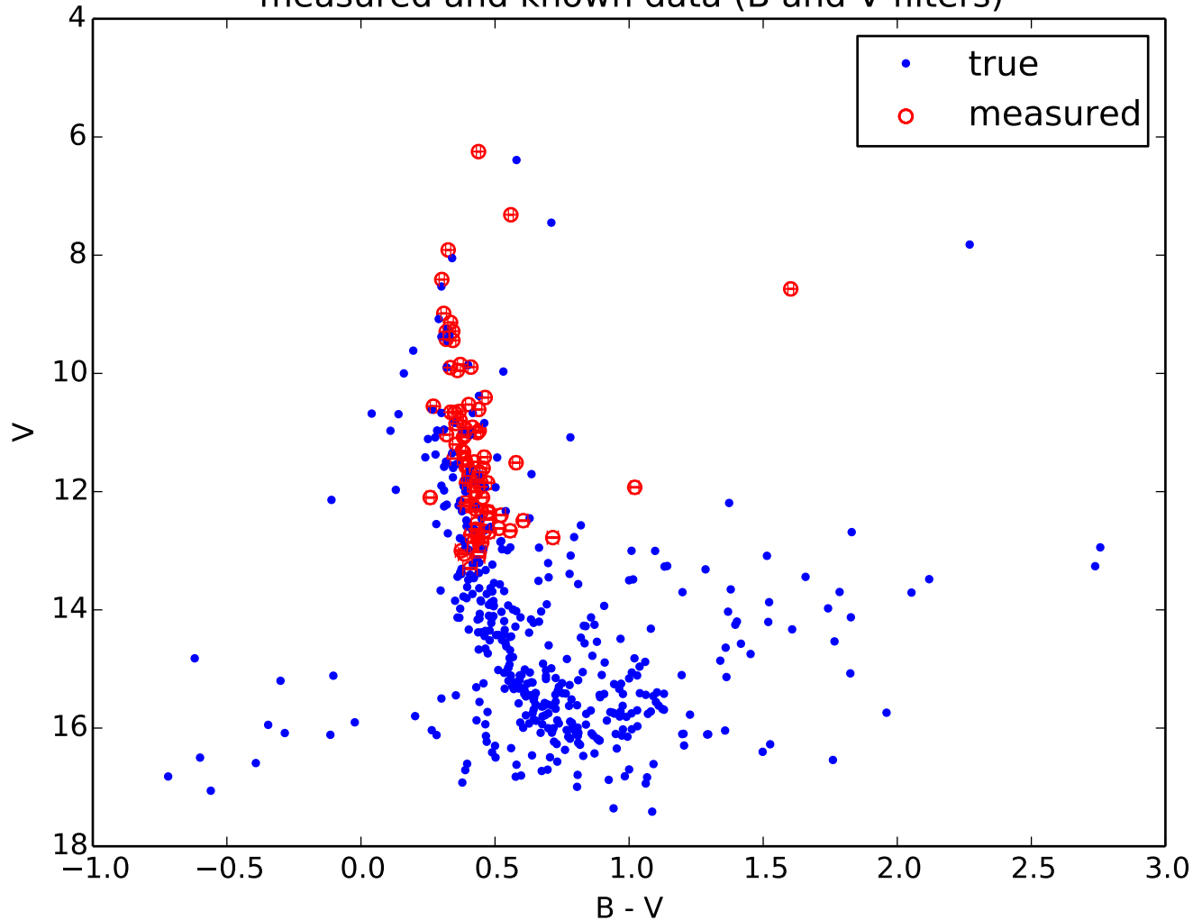
HR diagram for real Double Cluster stacked, comparing measured and known data (B and V filters)
